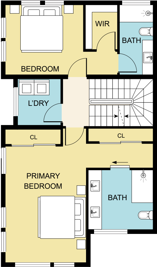
SECOND FLOOR
