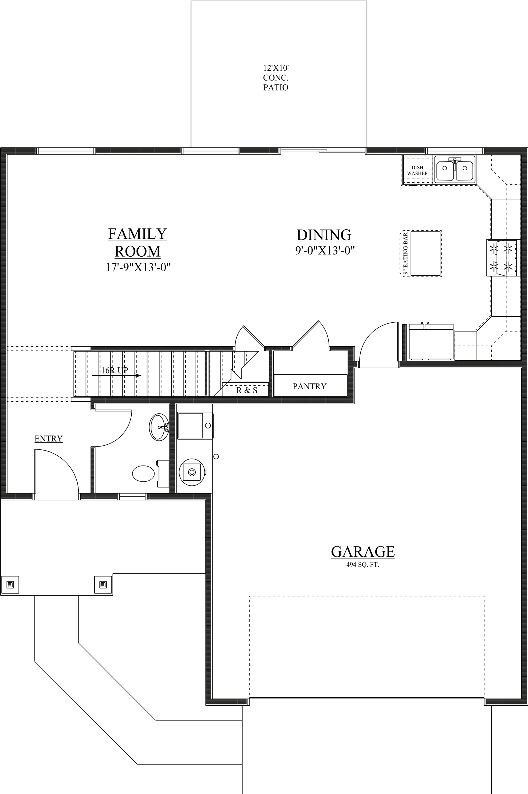
FLOOR PLAN
