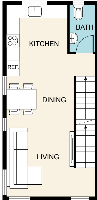
SECOND FLOOR
